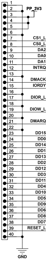
J1 FPC-1x40-P0.5mm-F2.0mm-S3.3mm-RL
